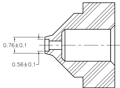
SECTION Z-Z
