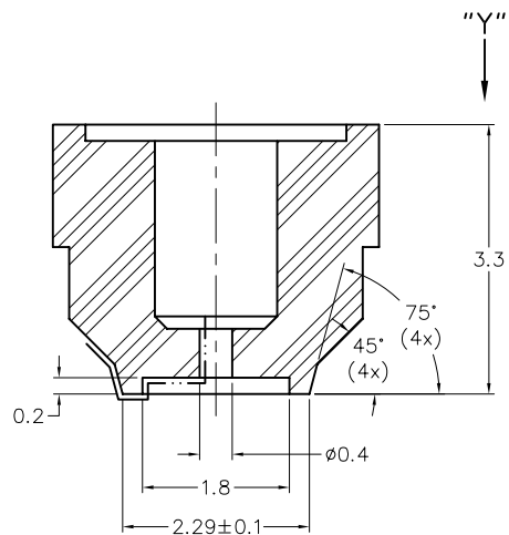
SECTION X-X
